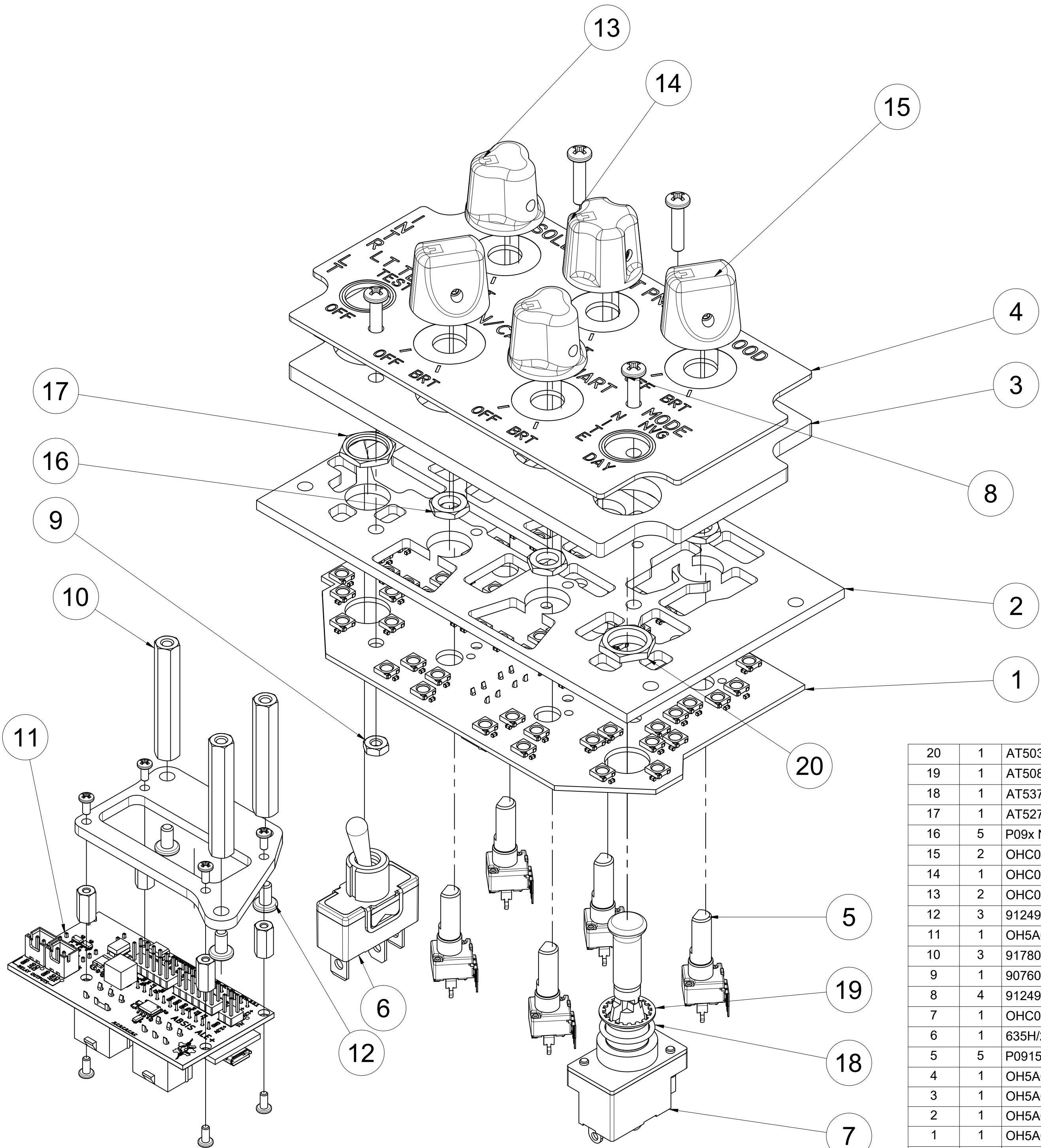
-1 ASSY SCALE 1.2:1
